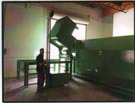
Side load carriage dumper dumping high volume autoclave carts into self-contained compactor.
