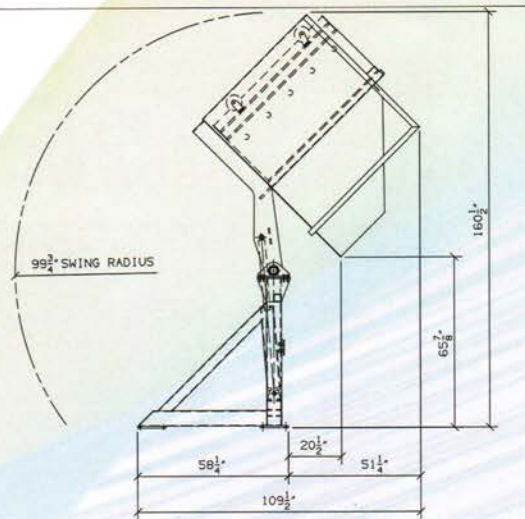
SIDE VIEW WITH CARRIAGE AT DUMPING POSITION
