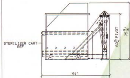
SIDE VIEW WITH CARRIAGE AT LOADING POSITION
